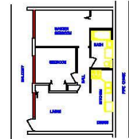
TYPICAL FLOOR PLAN (18 REQ'D) WHEELER TERRACE APTS
