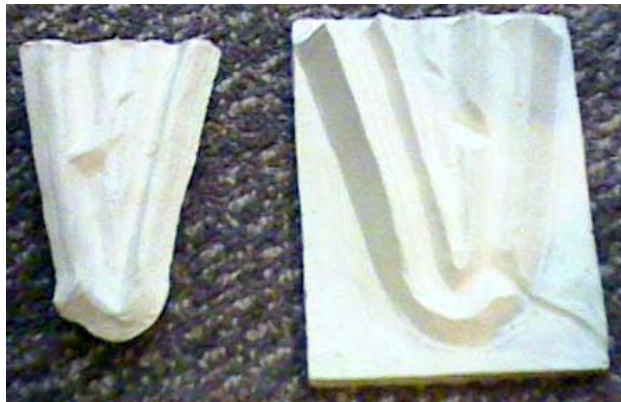
The third drawer also has a two-part model of an anticline to help show how what happens after weathering takes its toll on layers of rock.
